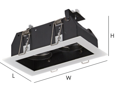
Model No: YZ5644 灯面尺寸 Lamp surface size: L173*W102mm 开孔尺寸 Hole size: Ø148*77mm 灯体高度 Height of lamp body: 84mm
