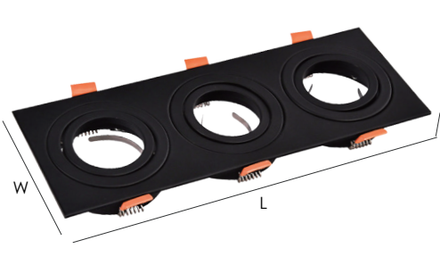
Model No: YZ5653-3 灯面尺寸 Lamp surface size: L260*W92mm 开孔尺寸 Hole size: Ø80mm 灯体高度 Height of lamp body: 25mm
