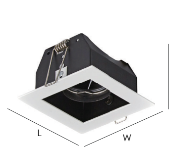
Model No: YZ5643 灯面尺寸 Lamp surface size: L102*W102mm 开孔尺寸 Hole size: Ø77*77mm 灯体高度 Height of lamp body: 84mm
