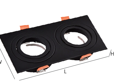
Model No: YZ5653-2 灯面尺寸 Lamp surface size: L174*W92mm 开孔尺寸 Hole size: Ø80mm 灯体高度 Height of lamp body: 25mm
