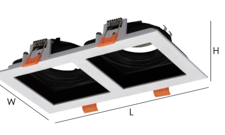
Model No: YZ5659-2 灯面尺寸 Lamp surface size: L185*W100mm 开孔尺寸 Hole size: Ø167*90mm 灯体高度 Height of lamp body: 32mm
