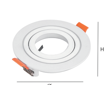
Model No: YZ5652 灯面尺寸 Lamp surface size: Ø92mm 开孔尺寸 Hole size: Ø75mm 灯体高度 Height of lamp body: 25mm
