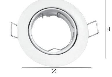
Model No: YZ5654 灯面尺寸 Lamp surface size: Ø92mm 开孔尺寸 Hole size: Ø78mm 灯体高度 Height of lamp body: 25mm
