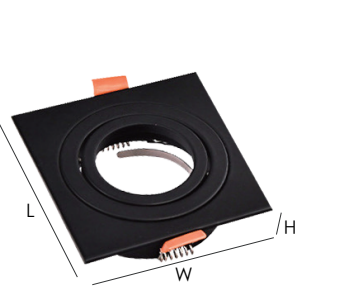
Model No: YZ5653 灯面尺寸 Lamp surface size: L92*W92mm 开孔尺寸 Hole size: Ø80mm 灯体高度 Height of lamp body: 25mm
