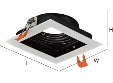
Model No: YZ5645 灯面尺寸 Lamp surface size: L119*W119mm 开孔尺寸 Hole size: Ø105mm 灯体高度 Height of lamp body: 37mm
