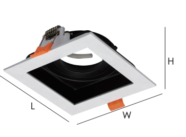
Model No: YZ5659 灯面尺寸 Lamp surface size: L100*W100mm 开孔尺寸 Hole size: Ø90mm 灯体高度 Height of lamp body: 32mm
