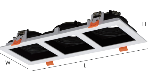
Model No: YZ5659-3 灯面尺寸 Lamp surface size: L270*W100mm 开孔尺寸 Hole size: Ø255*90mm 灯体高度 Height of lamp body: 32mm
